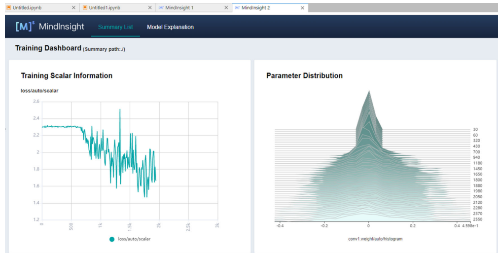
Figure 7-6 MindInsight page (3)
